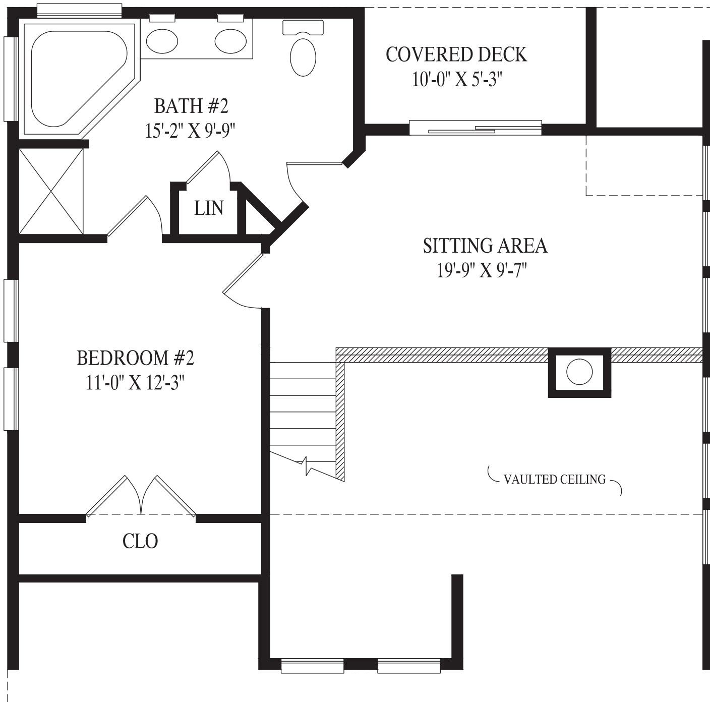
PIKE 530 Sq. Ft. PROPOSED SECOND FLOOR
