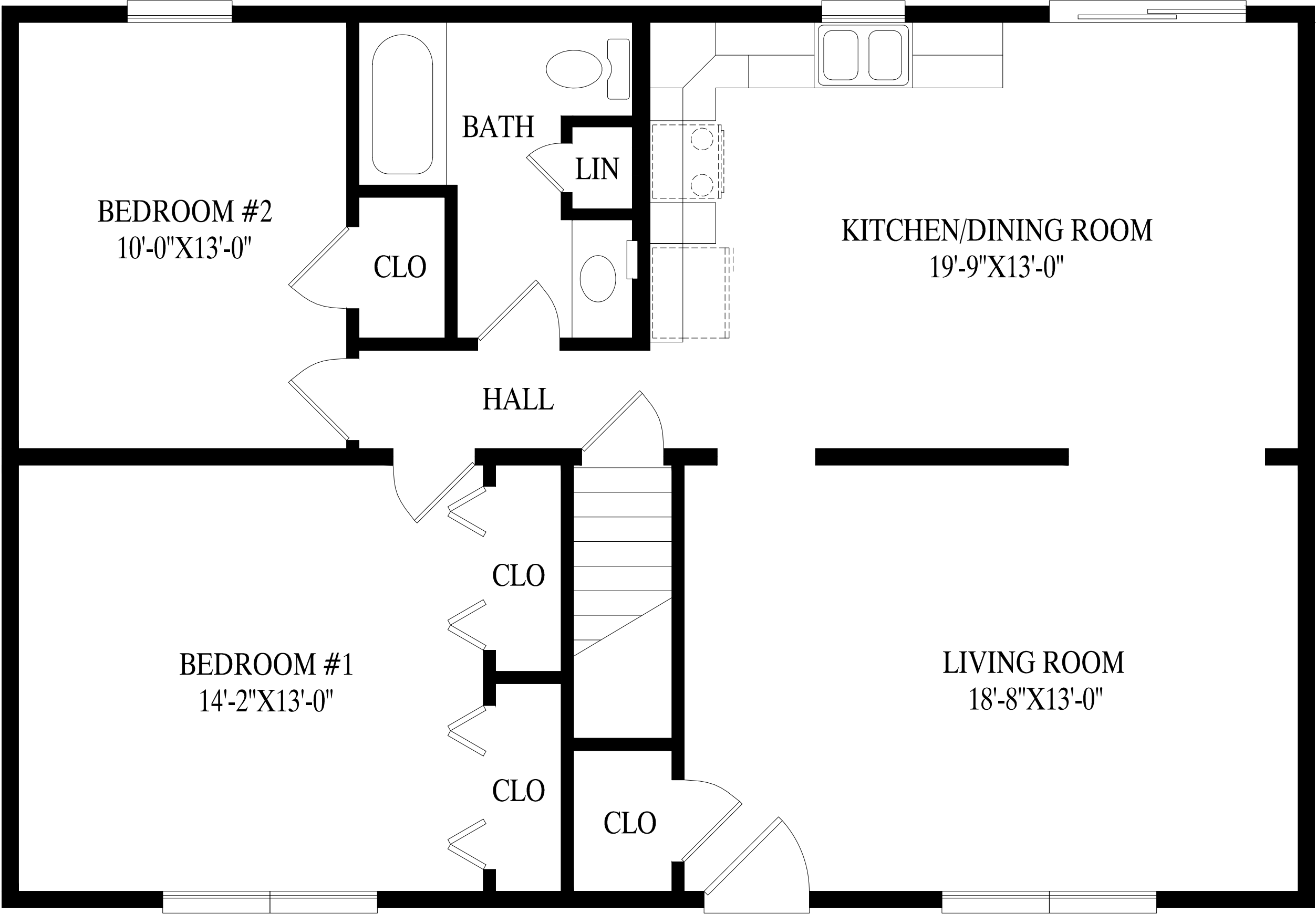
Oakwood 27' 6" X 40' Ranch 1100 Total Sq. Ft.
