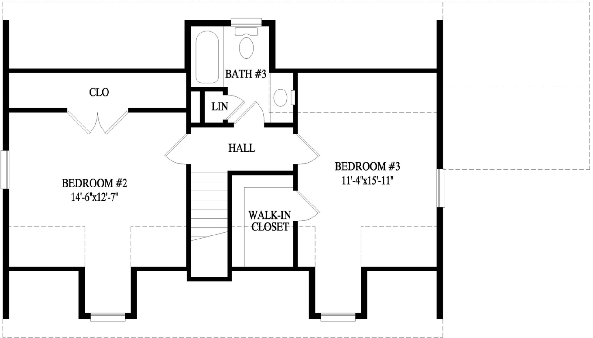
Proposed 2nd Floor - 667 sq. ft.
