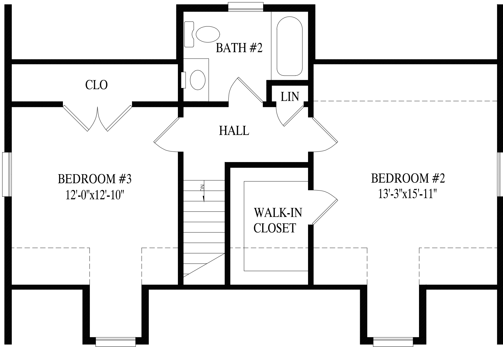
Proposed 2nd Floor - 674 sq. ft.
