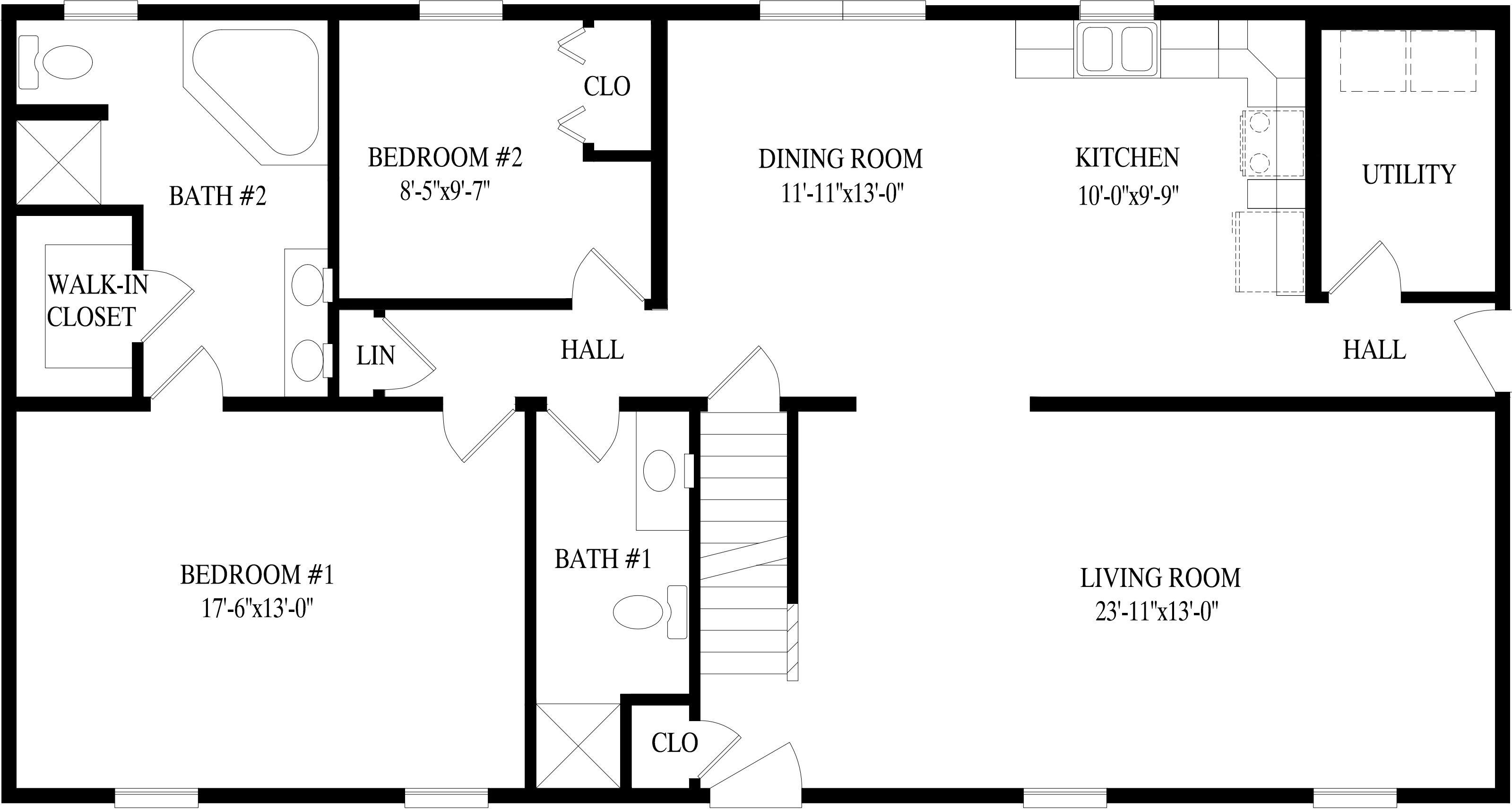
Huntington III 27' 6" X 48' Cape 1320 sq. ft. first floor
