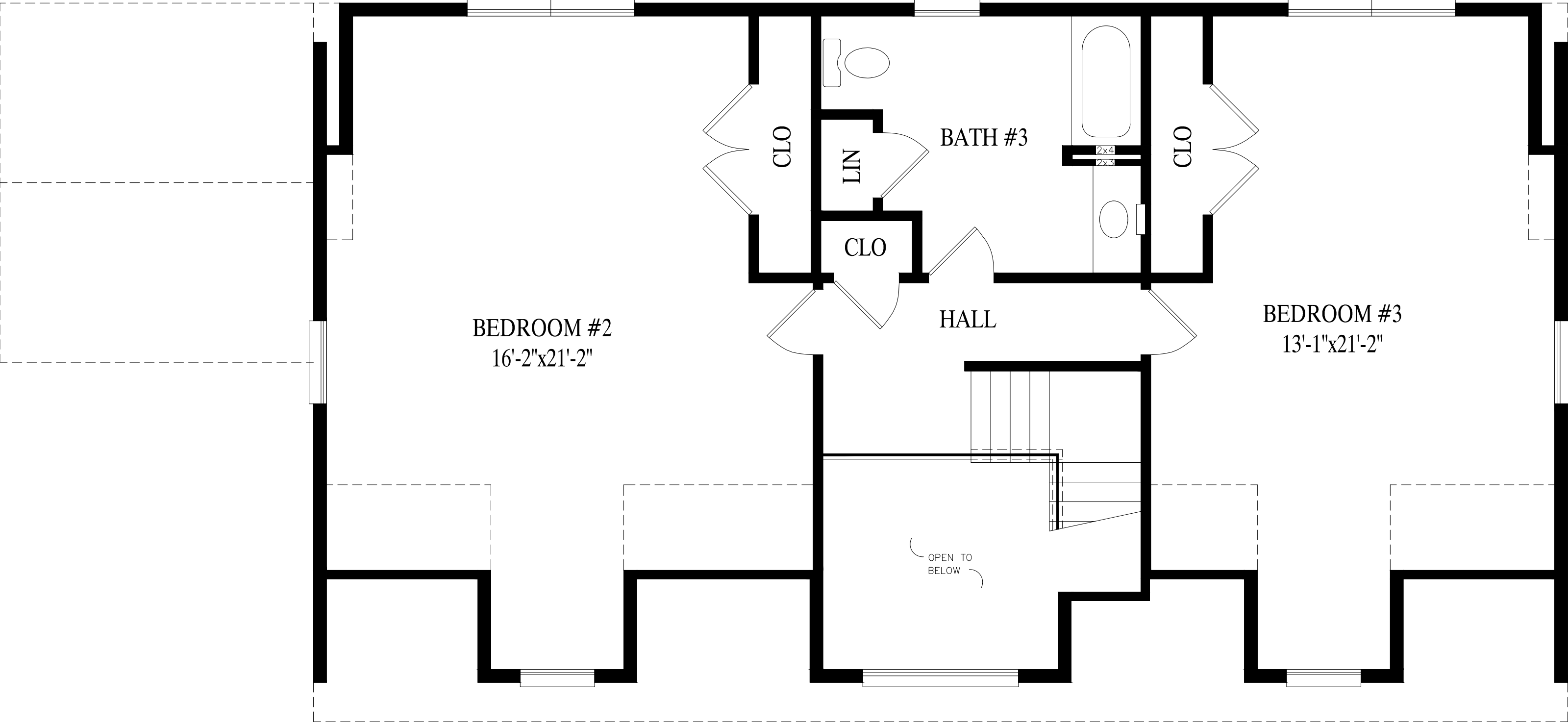
Proposed 2nd Floor - 1137 sq. ft.
